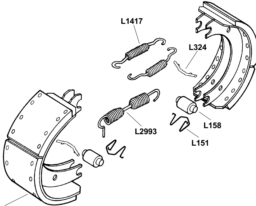
L3505 - Unlined FMSI 4693D (4")
