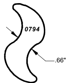
Second generation "Fast Rise" "0794" (July 1994) camshafts use the L158, 1-1/2" diameter cam roller. The cam S heads are marked 0794L or 0794R. Note the 0.66" distance across the S head. These must be used in pairs, LH and RH, on an axle. All retrofits from standard or first generation "Fast Rise" to the second generation "0794" must be done in pairs, LH and RH, on an axle to provide stable braking.
